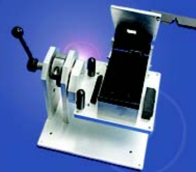
ASSEMBLY FIXTURES
