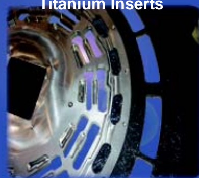
Selective Solder with Titanium Inserts
